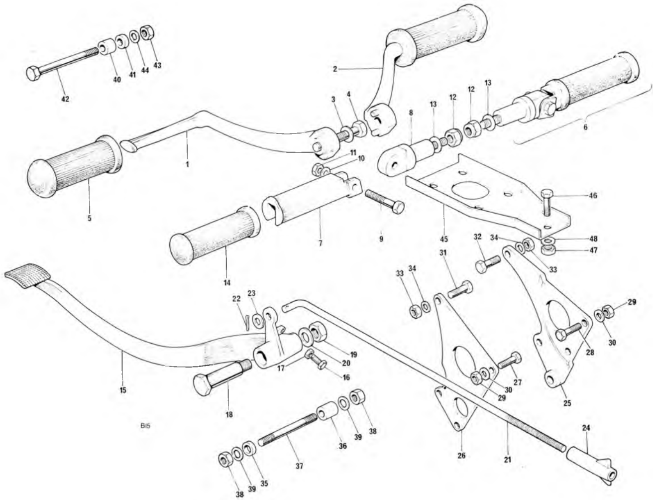
Fig. 16. MOTOR UNIT FITTING AND FOOTRESTS
