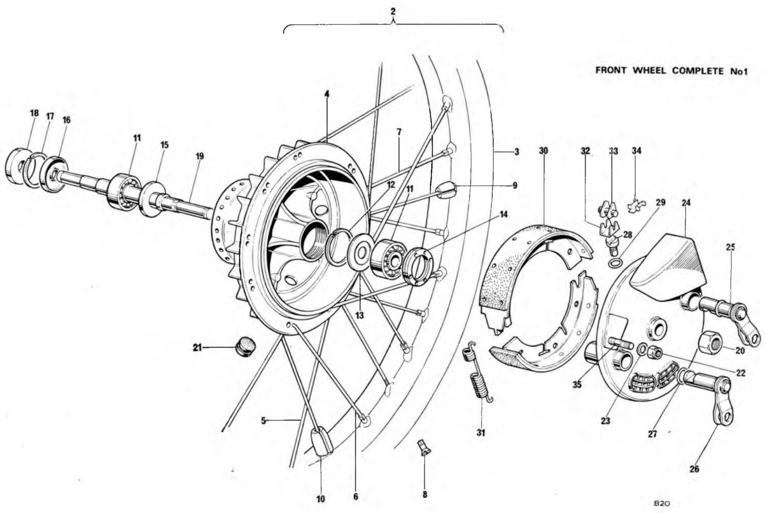
Fig. 21. FRONT WHEEL
