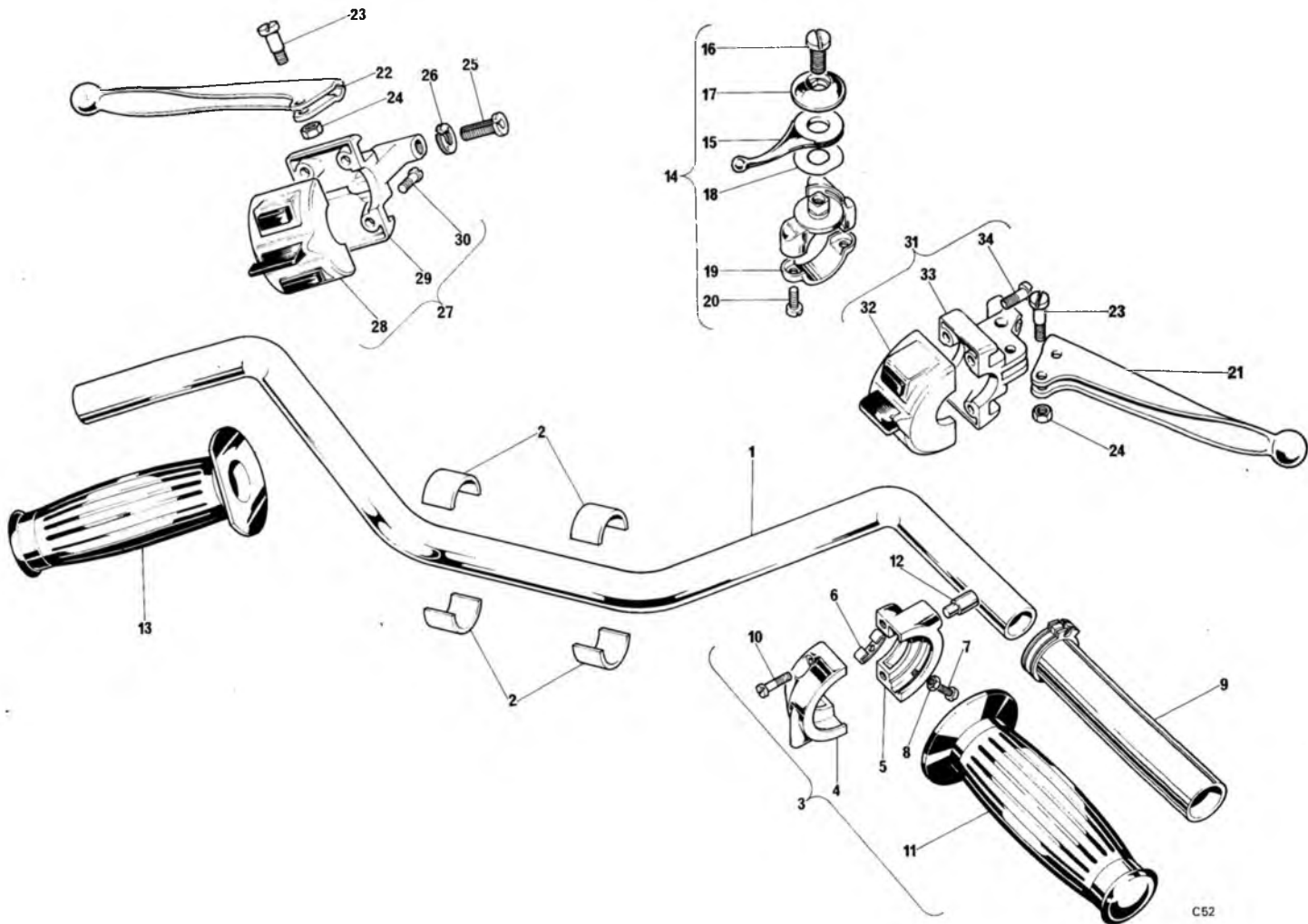
Fig. 26. HANDLEBAR AND CONTROL LEVERS
