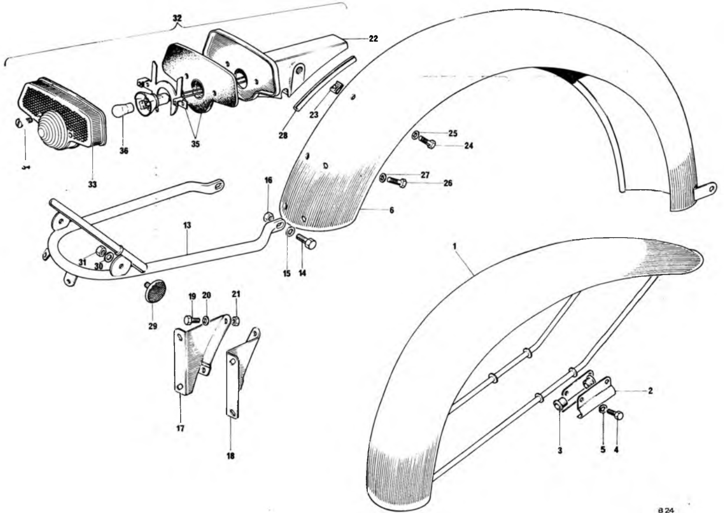
Fig. 25. FENDERS AND TAIL LAMP
