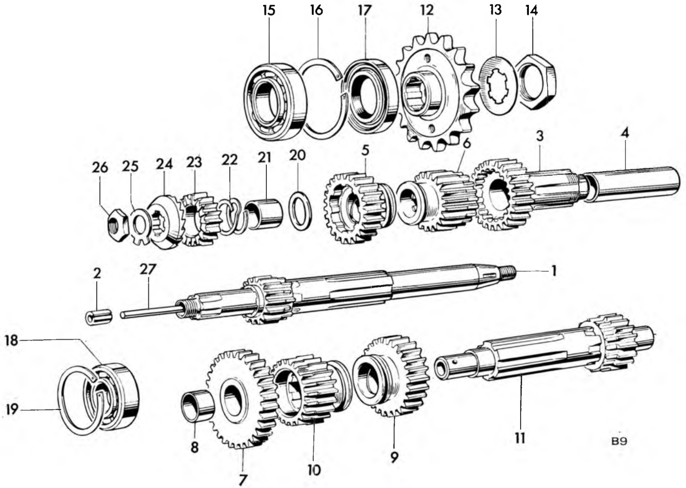
Fig. 10 GEARBOX SHAFTS AND GEARS
