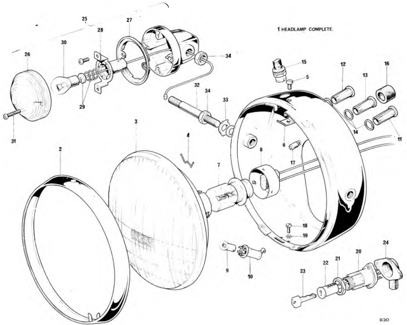
Fig. 31. HEADLAMP AND FLASHER LAMPS
