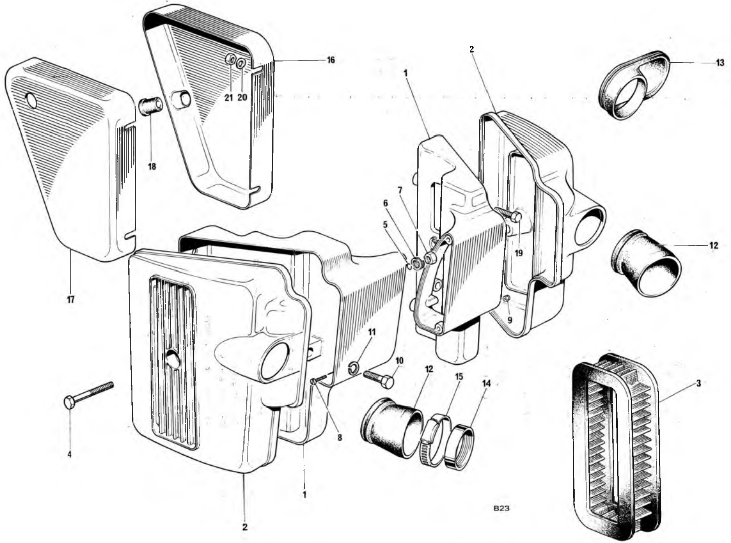
Fig. 24. AIR CLEANERS AND SIDE PANELS
