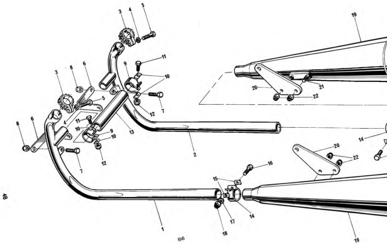
Fig. 17. EXHAUST PIPES AND MUFFLERS
