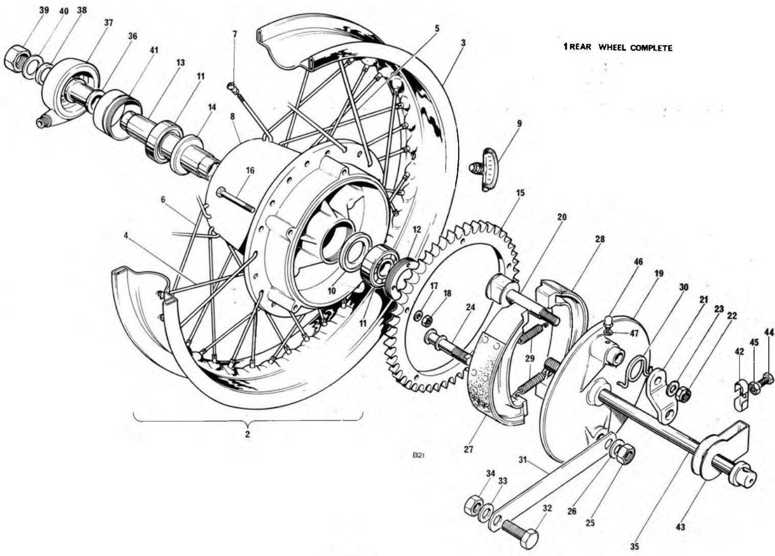
Fig. 22. REAR WHEEL
