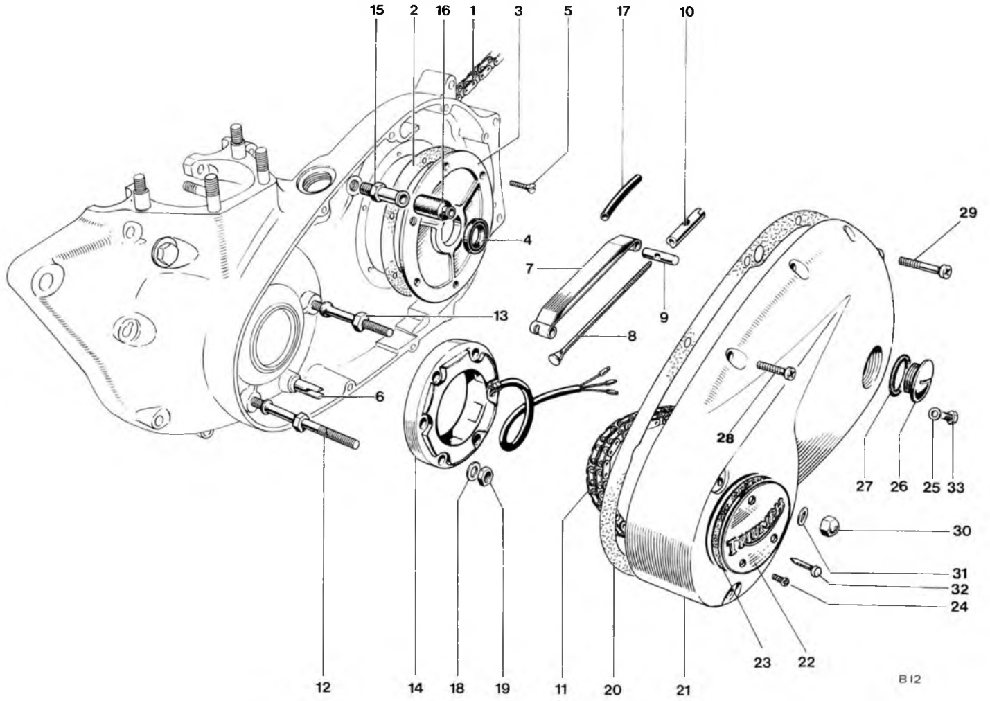
Fig. 13. CHAINCASE AND CHAINS
