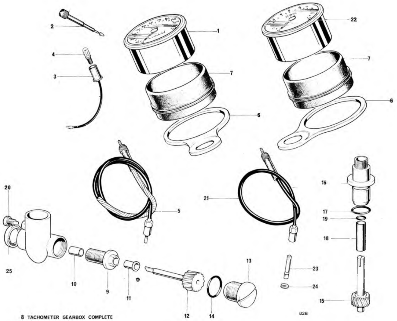
Fig. 29. SPEEDOMETER AND TACHOMETER
